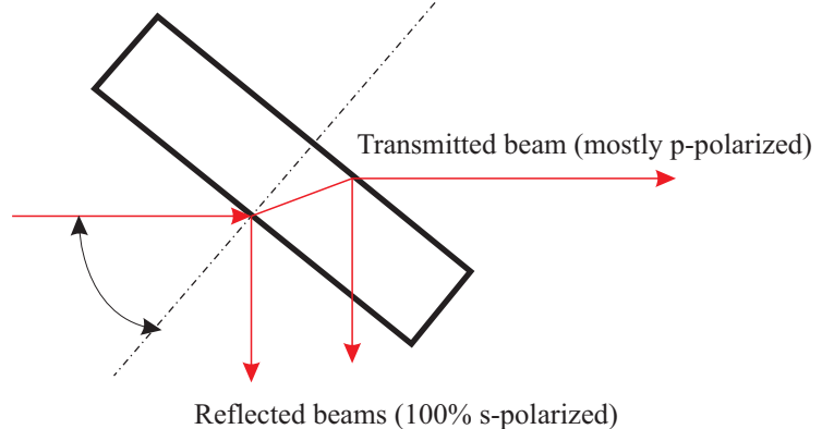
Fig.3 Brewster angle window.
