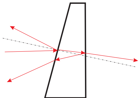
Fig. 2 A method to rid the optical system of unwanted reflections with using the wedge.
