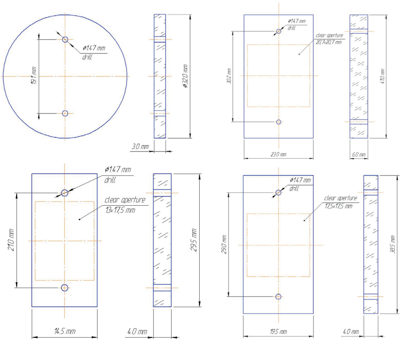
Fig. 1 Drawings of the drilled windows.
