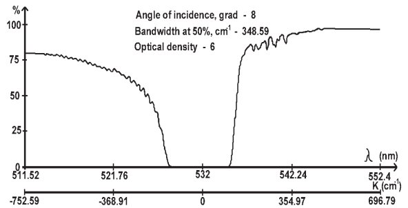
Fig. 1 Typical transmission curves of the Notch-4 filter for 633 nm and Narrow Notch-6 filter for 532 nm.
